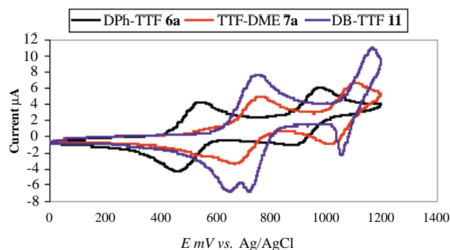
Figure 1. Cyclic voltammogram of DPh-TTF 6a , TTF-DME 7a , and DB-TTF 11 in CH 2 Cl 2 on a platinum electrode, concentration of (4.0x10 -5 M). Scan rate 200 mVs -1 , base-electrolyte TBAP 0.1 M.
